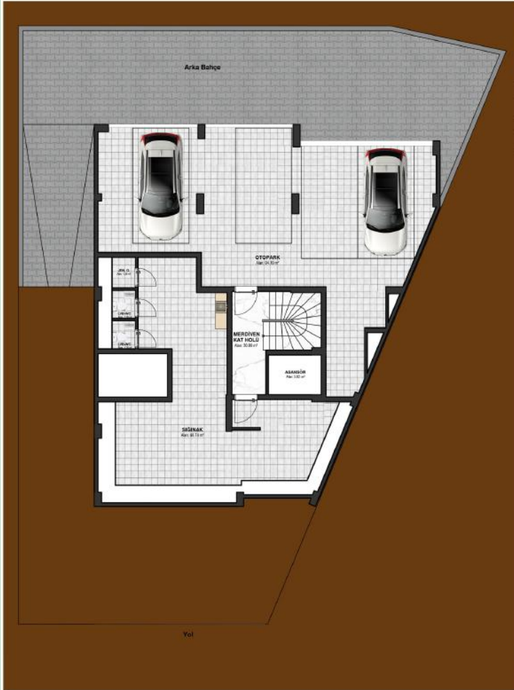
BODRUM KAT PLANI
